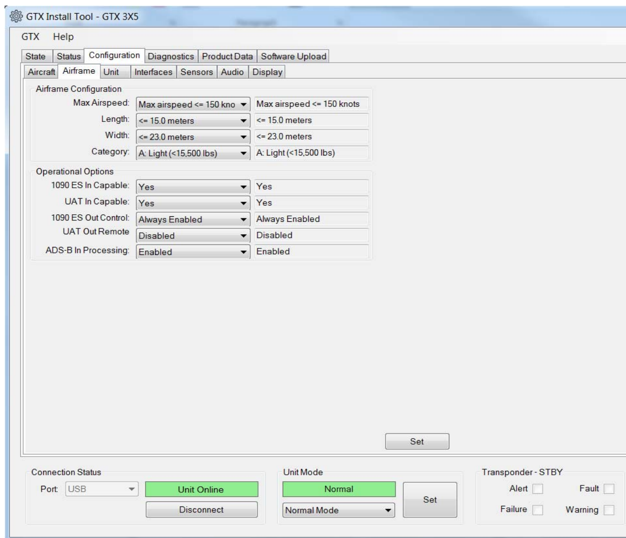
Figure 3-11 GTX 3X5 Configuration Group
