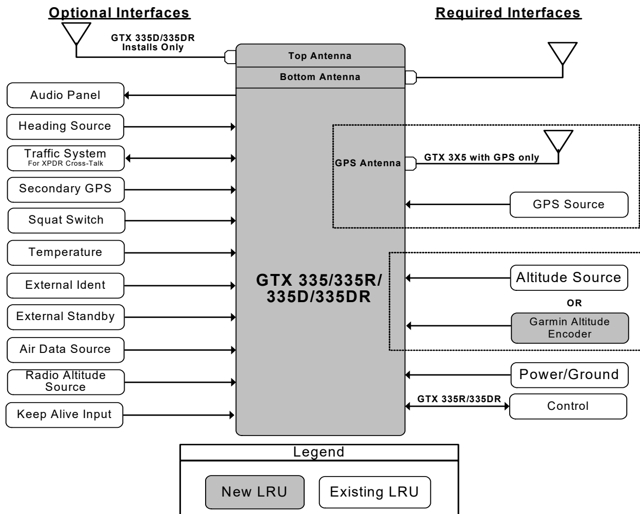
Figure 2-3 GTX 335/335D/335R/335DR Interface Summary
