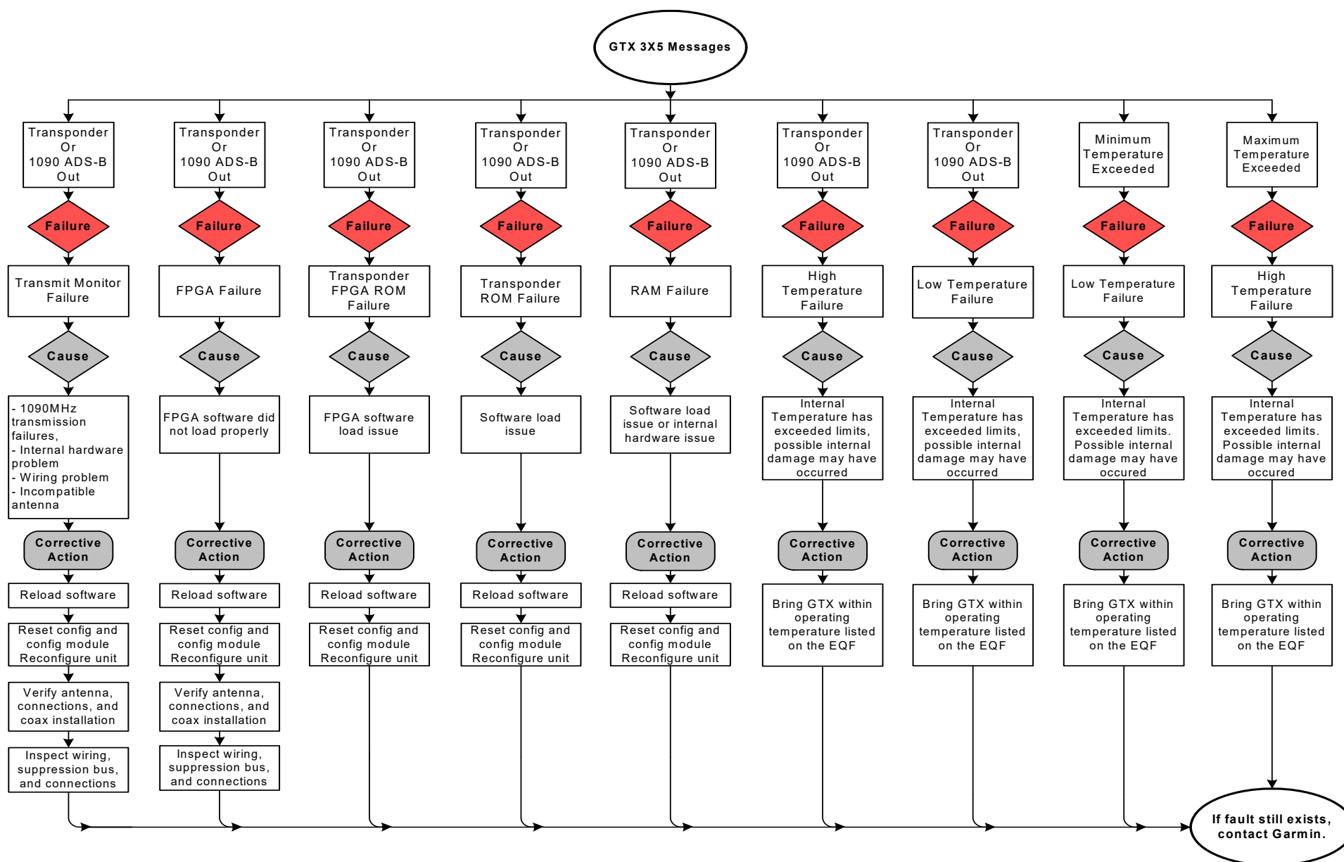
Figure 5-4 GTX 3X5 Transponder Alerts Sheet 2 of 5
