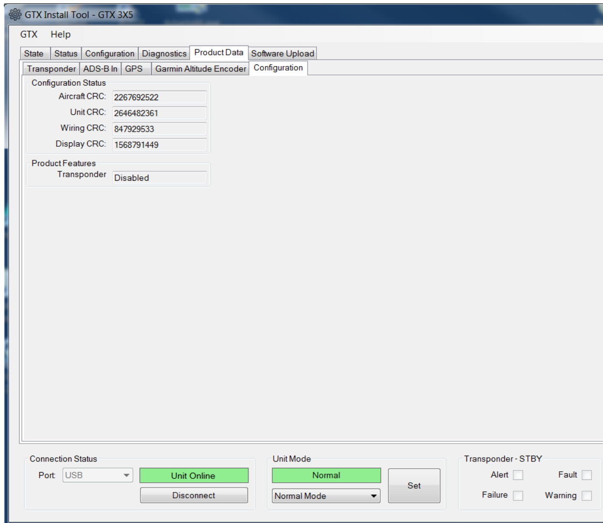
Figure 3-13 GTX 3X5 Product Data Group
